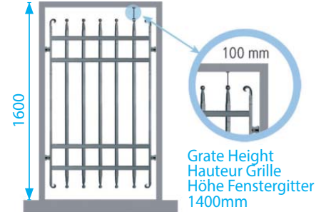
1400mm HIGH GRATE INSTALLATION ON A 1600mm HIGH WINDOW
