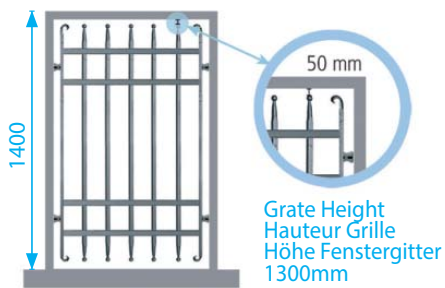
1300mm HIGH GRATE INSTALLATION ON A 1400mm HIGH WINDOW
