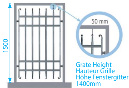
1400mm HIGH GRATE INSTALLATION ON A 1500mm HIGH WINDOW
